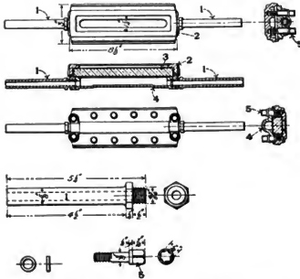
Figs. 3130-3140. Klinger Reflex Water Gage.
